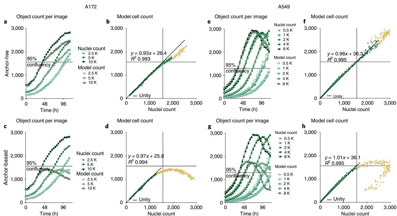
Fig. 4 | Validation of anchor-free and anchor-based model using fluorescent nuclei count. a–h, Predicted model counts are compared to fluorescence nuclei counts on A172 and A549 cells. Time course graphs show per-image object counts across different cell seeding densities over time for fluorescent nuclei and the models for the anchor-free ( a ) and anchor-based ( c ) model for A172 cells and the anchor-free ( e ) and anchor-based ( g ) model for A549 cells. Correlation plots for each image show R^2 > 0.99 with a gradient close to 1 when comparing nuclei count and label-free predictions of the anchor-free ( b ) and anchor-based ( d ) models for A172 cells and anchor-free ( f ) and anchor-based ( h ) models for A549 cells. The yellow markers highlight data removed from the correlation calculations. On all graphs, the dotted line represents the 95% cell confluence level. Data are shown as mean \pm s.e.m. for n = 4 images ( a,c ) and n = 3 images ( e,g ).
