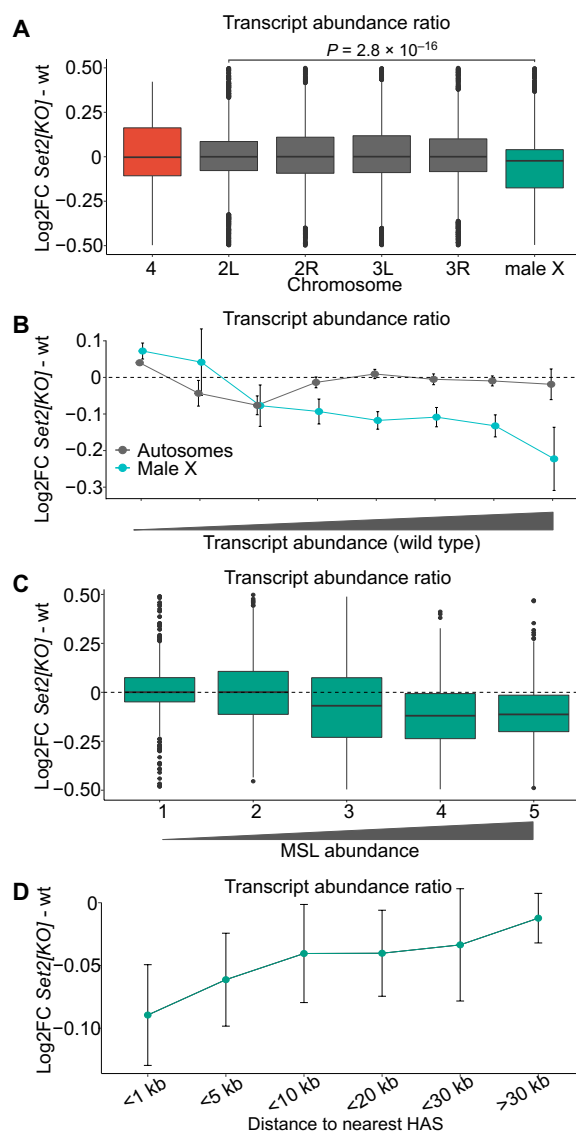
Fig. 2. Set2 is required for balanced transcription output from the single male X chromosome. (A) Box plots of chromosome-specific transcript abundance ratios ( \log_2 fold change) between Set2 1 and wild type for chromosome 4 (red), X chromosome (green), and the autosome arms (gray). The abundance of transcripts from X chromosome of the Set2 1 mutant is significantly reduced as compared to the autosomes. The likelihood that observed differences are due to chance was evaluated by unpaired two-sample Wilcoxon tests comparing values for the X chromosome and chromosome arm 2L (the most similar autosome arm). (B) Transcript abundance in Set2 1 versus wild type plotted as fold change ( \log_2 ). Genes were binned according to Flybase RNA-seq expression level intervals. The X chromosome genes with higher transcriptional output in the wild type are significantly more affected compared to those on autosomes. (C) Box plots of average transcript abundances of the X-chromosomal genes in Set2 1 versus wild type. The genes are grouped in equally sized bins based on their MSL1-binding strength; 1 (lowest) to 5 (highest). Genes with higher MSL1 levels show greater fold change compared to genes with no or low amounts of MSL1 bound. (D) Average \log_2 fold change for X-chromosomal genes binned by distance to HASs. In (B) and (D), the error bars indicate the 95% confidence intervals.
