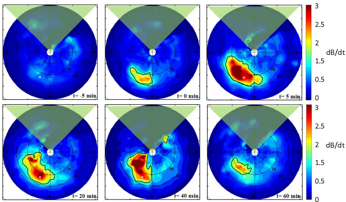
Fig. 8. Two dimensional superposed epoch analysis of the 95 % percentile of the 81 substorms Each panel is in a magnetic coordinate system with 12 magnetic local time (MLT) at the top, 00 MLT at the bottom, 06 MLT on the right, and 18 MLT on the left. From epoch time 0 min (substorm onset) to epoch time 60 min, the area dB/dt that exceeds 1.5 nT/s (black contour in pre-midnight sector) covers a large portion of the pre-midnight sector.
