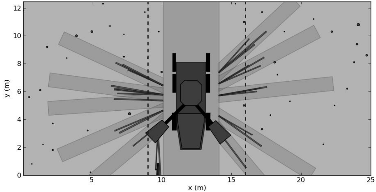
Figure 1. The double-crane harvester concept simulated with the limits for the stochastic strip-road (vertical dashed lines).
