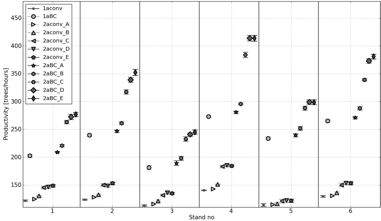
3 Figure 2. Simulated productivity for the different machine types and automation configurations (A - E) (see Table 2) and six different stands (1 - 6) with 95% confidence intervals. 1a/2a means one or two arms, BC is boom-corridor head and Conv is the conventional crane head.
