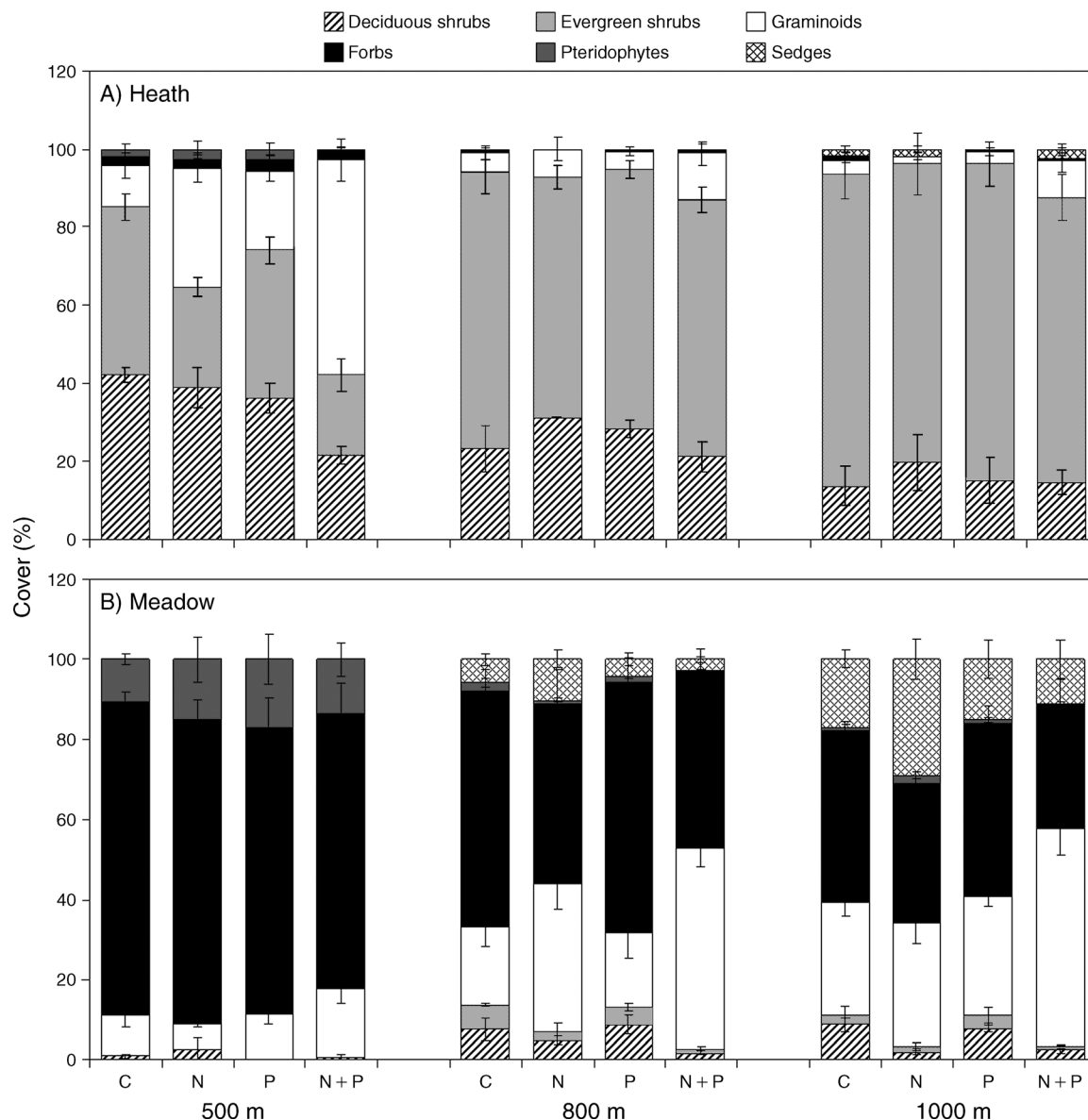
Fig. 2. The mean percentage cover ( \pm SE) of plant functional groups in plots without fertilizer addition (Control) or amended with N, P, or N + P for (A) subarctic heath and (B) meadow along an elevational gradient. ANOVA results are given in Appendix B, and actual values with SEs are given in Appendix C.
